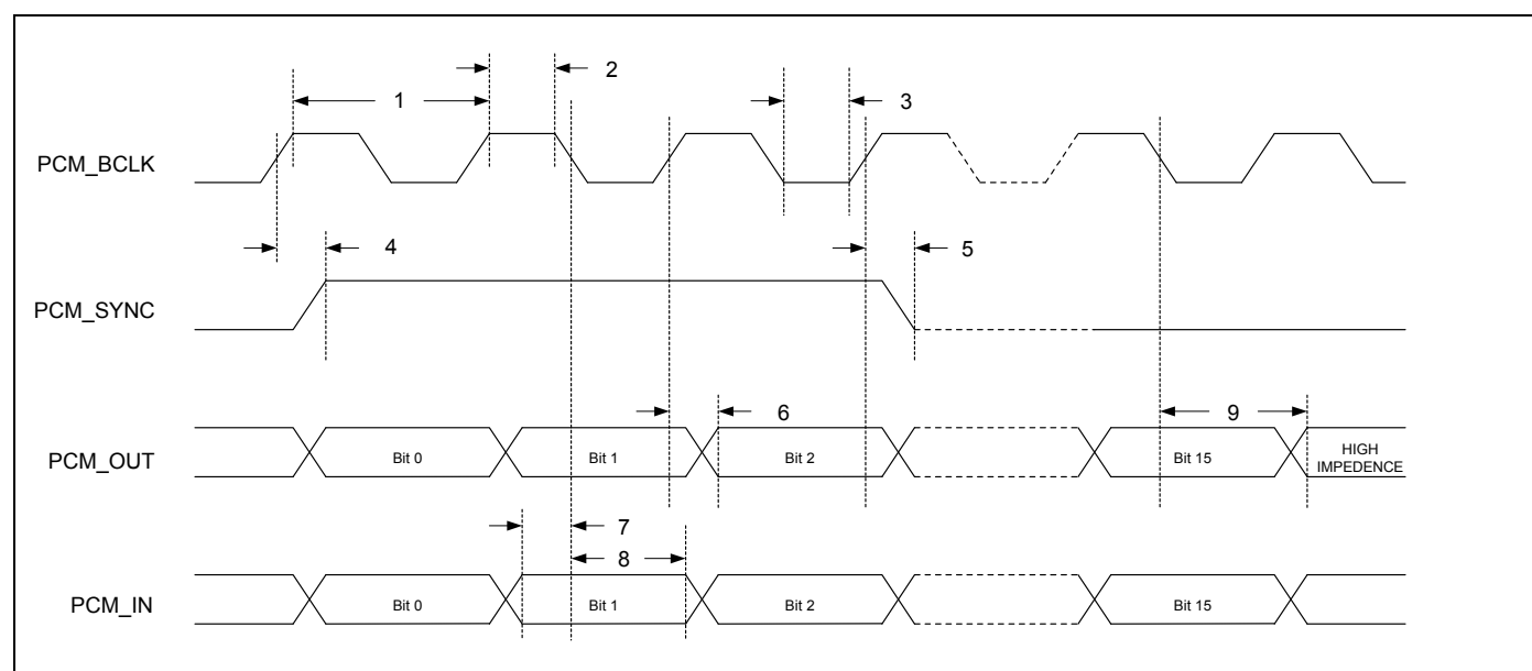
Figure 15. PCM Interface Timing (Long Frame Synchronization, Master Mode)
