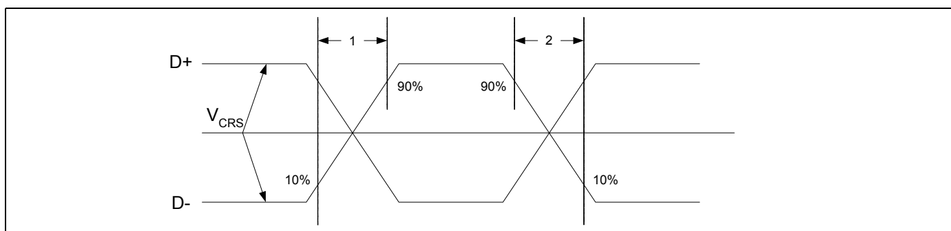
Figure 11. USB Full-Speed Timing
