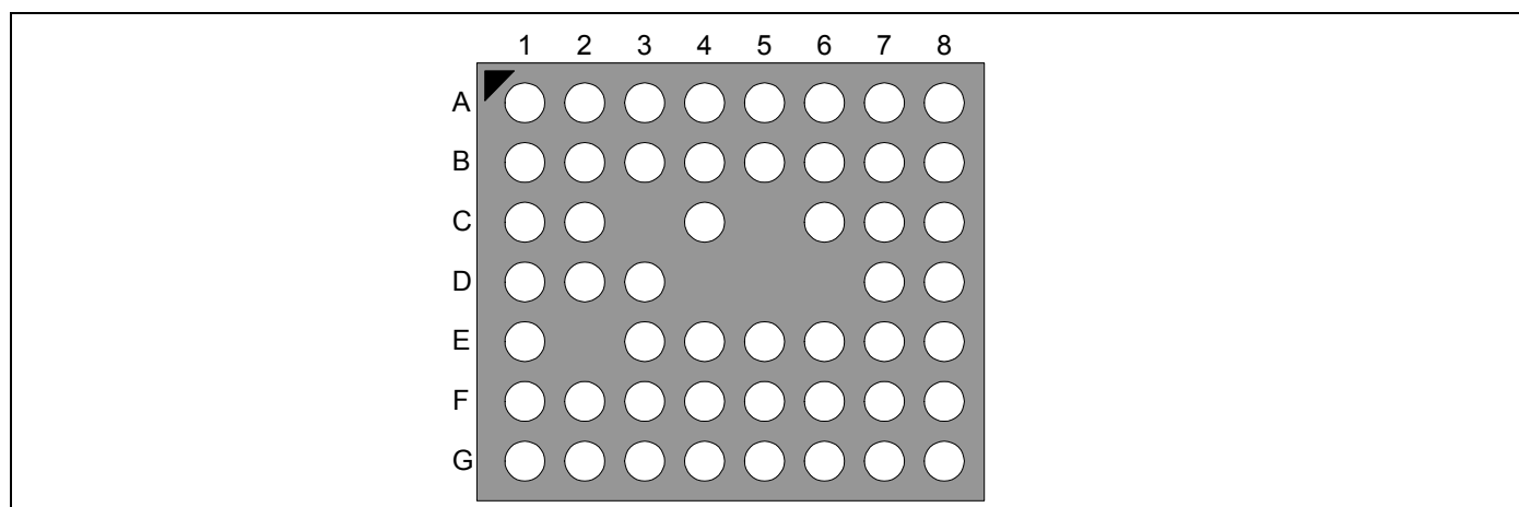
Figure 9. 4.5 x 4 x 0.8 mm (WFBGA) Array
