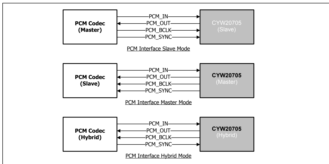
Figure 5. PCM Interface with Linear PCM Codec
