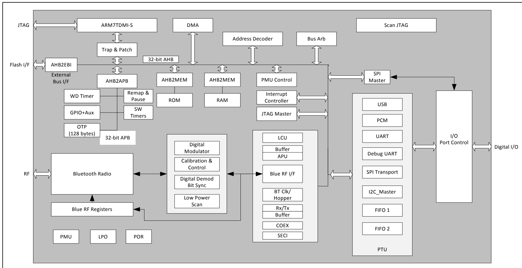
Figure 2. Functional Block Diagram
