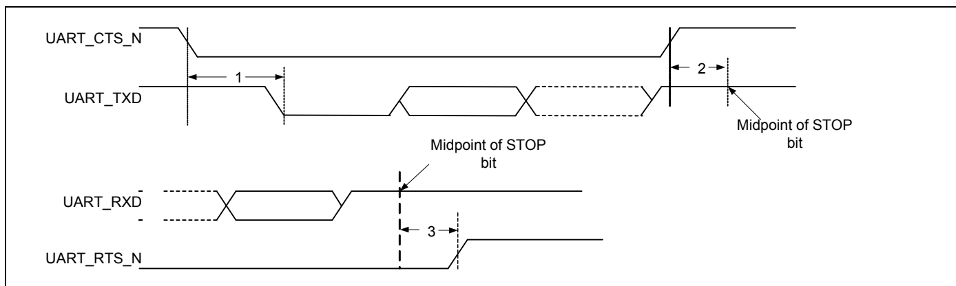
Figure 12. UART Timing
