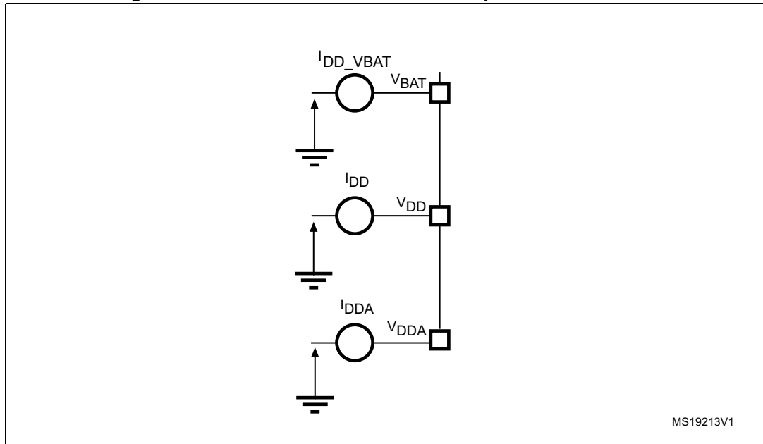
Figure 11. Scheme of the current-consumption measurement
