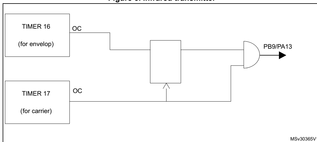
Figure 3. Infrared transmitter
