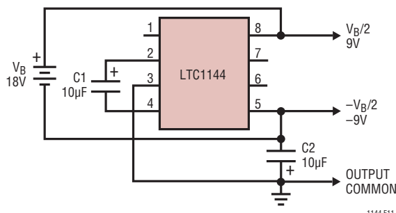
Figure 11. Battery Splitter
