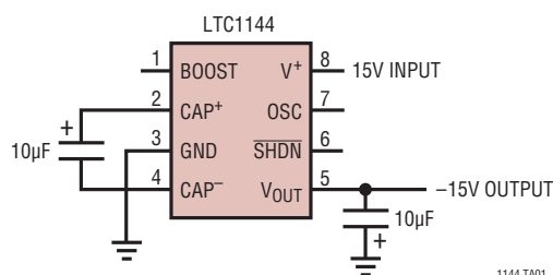
Generating -15V from 15V
