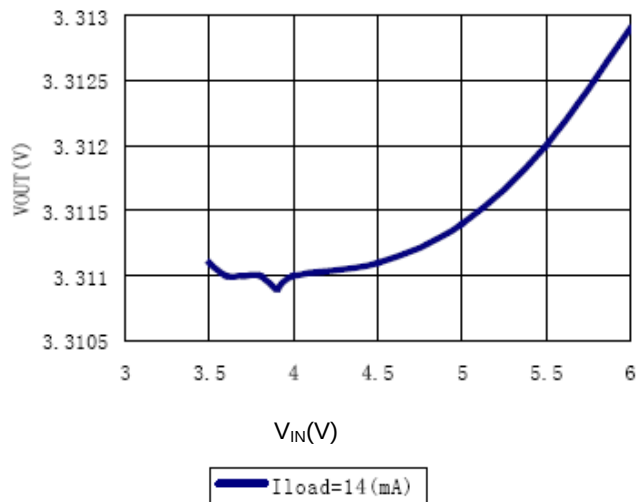
Lin Regulation
