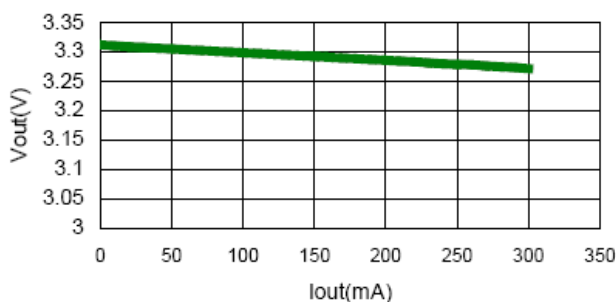
Load Regulation ( V_{\text{out}}=4.5\text{V} )
