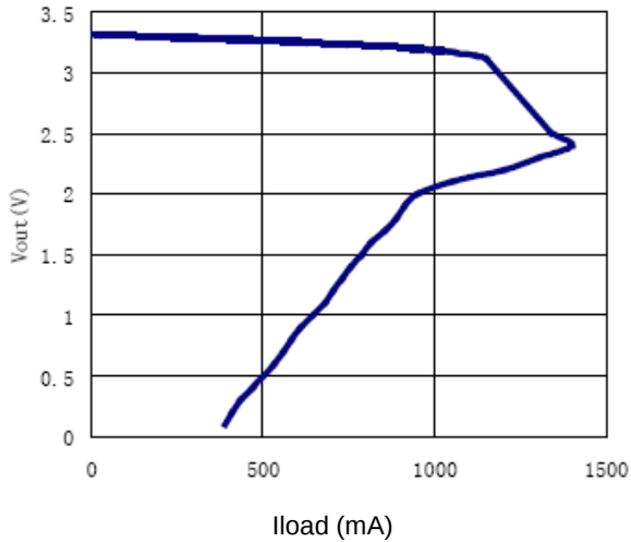
Current limit vs. Vout
