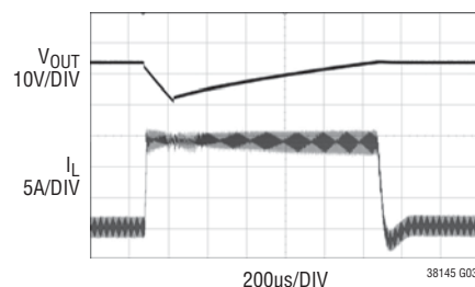
Overcurrent Operation
