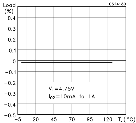
Figure 9: Reference Load Regulation vs Temperature
