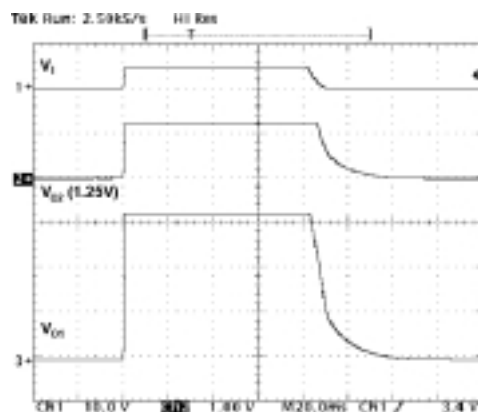
Figure 33: Start-Up Transient
