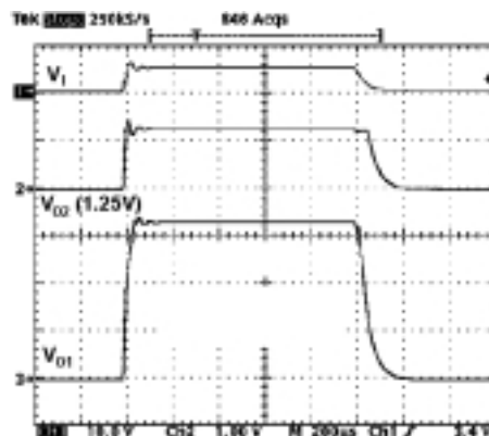
Figure 34: Start-Up Transient
