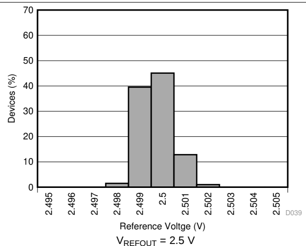
图 48. Reference Voltage Histogram
