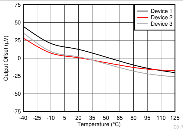
图 21. Shunt-Sense Amplifier Output Offset vs Temperature
