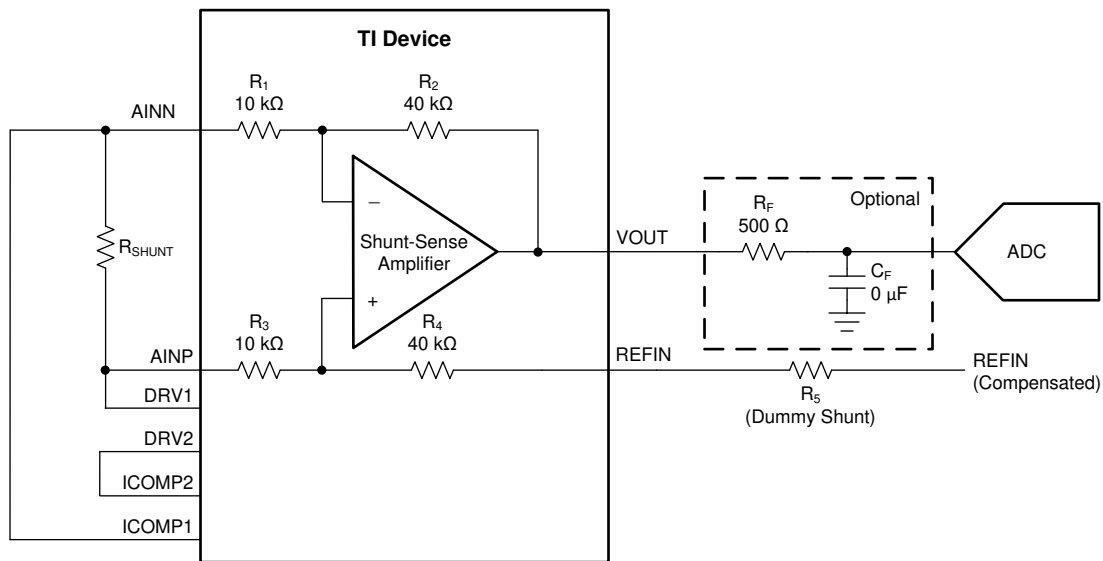
图 65. Internal Difference Amplifier With an Example of a Decoupling Filter
