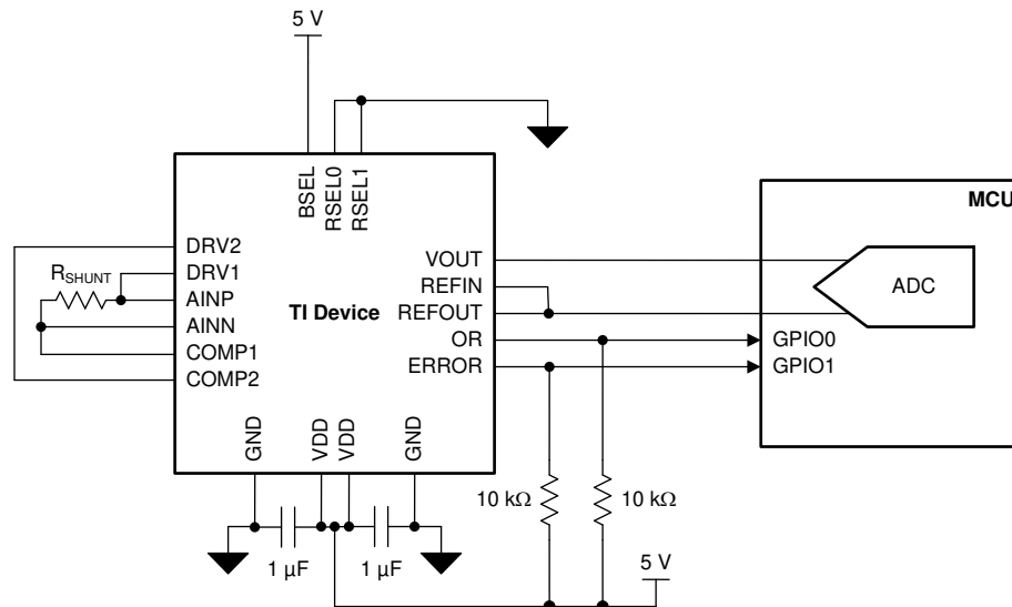
图 67. Linear-Position Sensing
