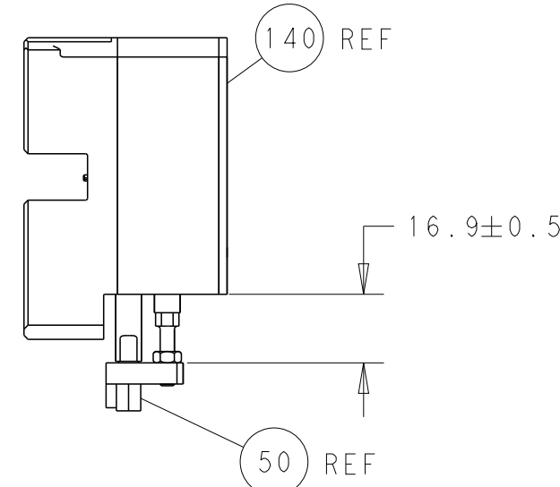
HOLDDOWN SET-UP
