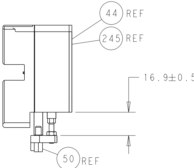
HOLDDOWN SET-UP
