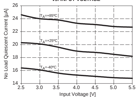
NO LOAD QUIESCENT CURRENT vs. INPUT VOLTAGE
