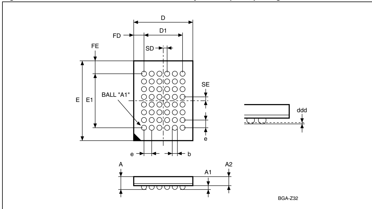
Figure 19. TFBGA48 6x8mm - 6x8 active ball array, 0.8mm pitch, package outline
