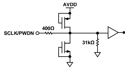
Figure 32. Equivalent SCLK or PDWN Input Circuit
