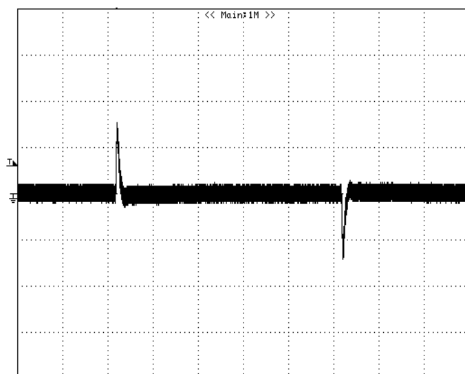
Figure 20: Typical transient response to step load change at 1A/μS from 100%~ 50%~100% of I_o , max at 12Vin, 3.3Vout ( C_{out} = 1\mu F ceramic, 47μF+10μFceramic) CH1 : VOUT, 0.1V/div, 200μS/div
