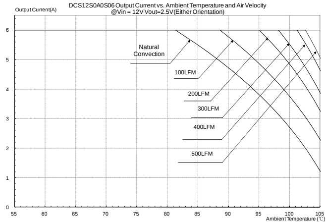
Figure 44: Output current vs. ambient temperature and air velocity@ V_{in}=12V , V_{out}=2.5V (Either Orientation)
