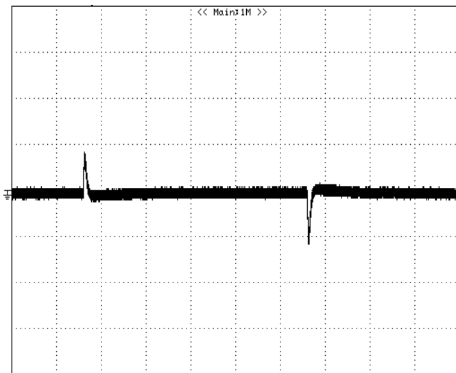
Figure 22: Typical transient response to step load change at 1A/\mu S from 100%~ 50%~100% of I_o , max at 12Vin, 1.8Vout (Cout = 1uF+ 47uF+10uF ceramic) CH1 : VOUT, 0.1V/div,200uS/div
