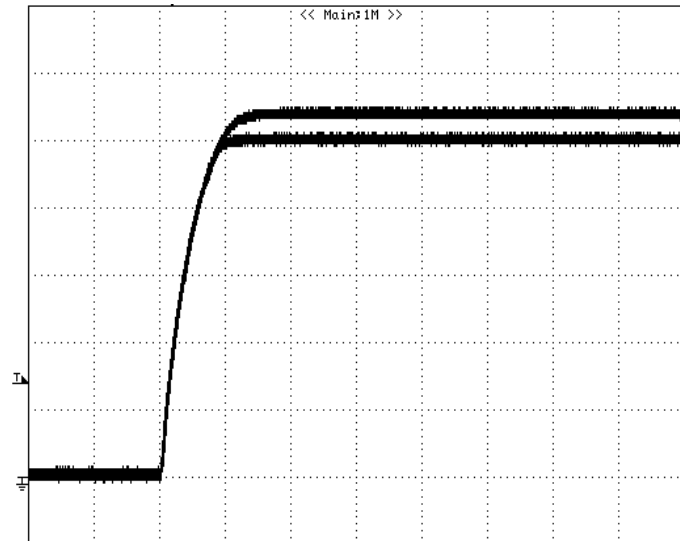
Figure 27: Tracking function, Vtracking=5.5 V, Vout= 5.0V, full load Top trace:Vtracking, 1V/div; Bottom trace: Vout,1 V/div;1ms/div
