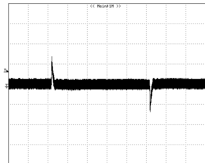
Figure 19: Typical transient response to step load change at 1A/μS from 100%~ 50%~100% of I_o , max at 12Vin, 5.0Vout ( C_{out} = 1\mu F ceramic, 47μF+10μFceramic) CH1 : VOUT, 0.1V/div, 200μS/div
