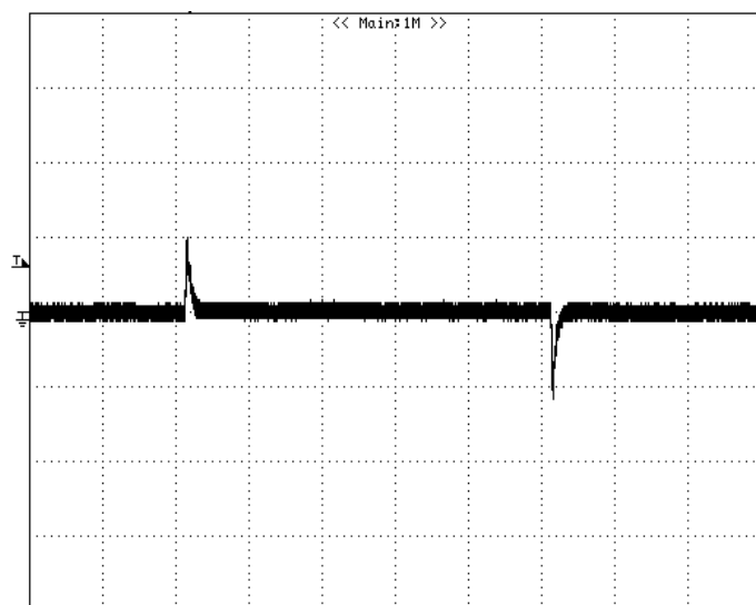
Figure 23: Typical transient response to step load change at 1A/\mu S from 100%~ 50%~100% of I_o , max at 12Vin, 1.2Vout (Cout = 1uF+ 47uF+10uF ceramic) CH1 : VOUT, 0.1V/div, 200uS/div
