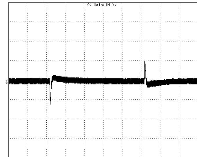
Figure 21: Typical transient response to step load change at 1A/\mu S from 100%~ 50%~100% of I_o , max at 12Vin, 2.5Vout (Cout = 1uF+ 47uF+10uF ceramic) CH1 : VOUT, 0.1V/div, 200uS/div
