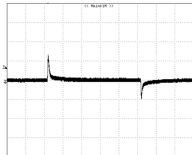
Figure 24: Typical transient response to step load change at 1A/\mu S from 100%~ 50%~100% of I_o , max at 12Vin, 0.59Vout (Cout = 1uF+ 47uF+10uF ceramic) CH1 : VOUT, 0.1V/div, 200uS/div
