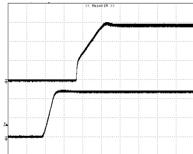
Figure 18: Turn on delay time at 12Vin, 0.59V/6A out (Top trace: VOUT, 0.2V/div; Bottom trace: VIN, 5V/div; 2mS/div)
