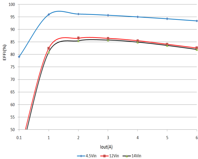
Figure 5: Converter efficiency vs. output current (1.2Vout)
