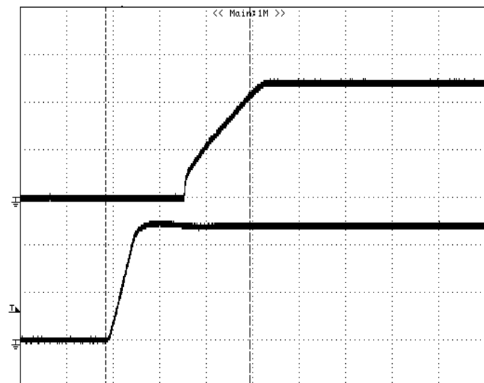
Figure 17: Turn on delay time at 12Vin, 1.2V/6A out (Top trace: VOUT, 0.5V/div; Bottom trace: VIN, 5V/div; 2mS/div)
