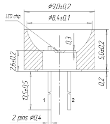
1 - LED cathode 2 - LED anode
