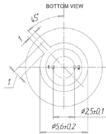
(Unit: mm)
