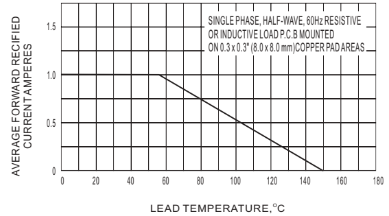
FIG.2 MAXIMUM AVERAGE FORWARD CURRENT DERATING
