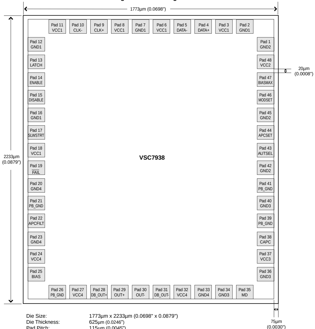
Figure 1: Pad Assignments
