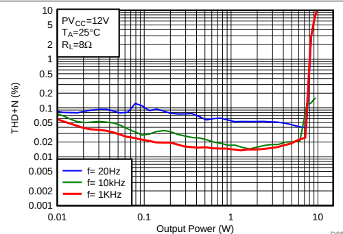
图 35. THD+N vs Output Power
