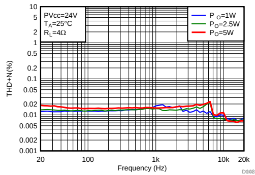
图 135. THD+N vs Frequency
