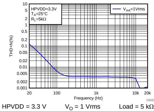
图 59. THD+N vs Frequency
