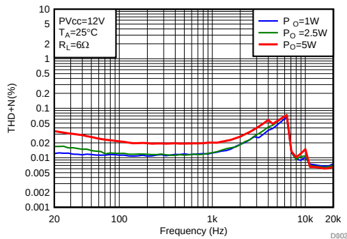
图 128. THD+N vs Frequency (1 SPW Mode, PVDD = 12 V, Load = 6 \Omega , BTL Mode)
