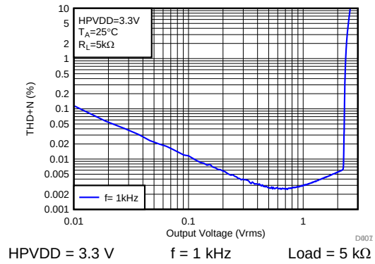
图 60. THD+N vs Output Voltage
