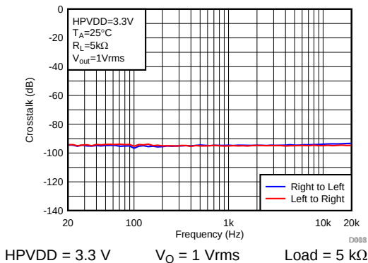
图 61. Crosstalk vs Frequency
