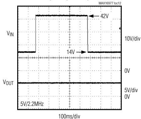
LOAD DUMP TEST
