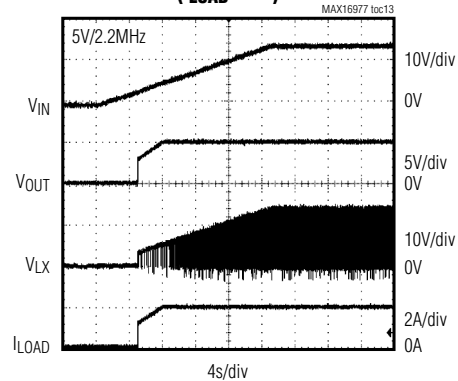
OUTPUT RESPONSE TO SLOW INPUT RAMP ( I_{LOAD} = 2A )
