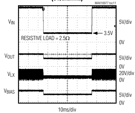
UNDERVOLTAGE PULSE (5V/2.2MHz)
