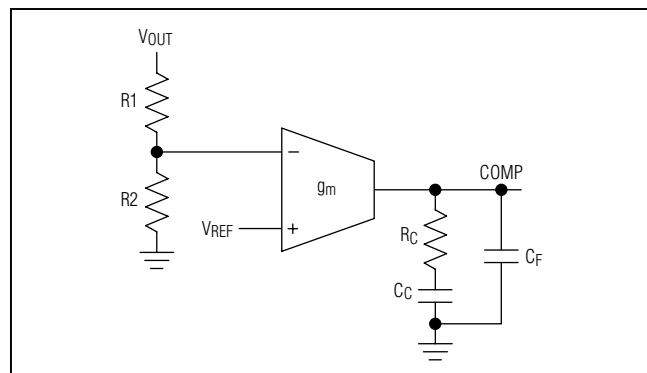
Figure 3. Compensation Network
