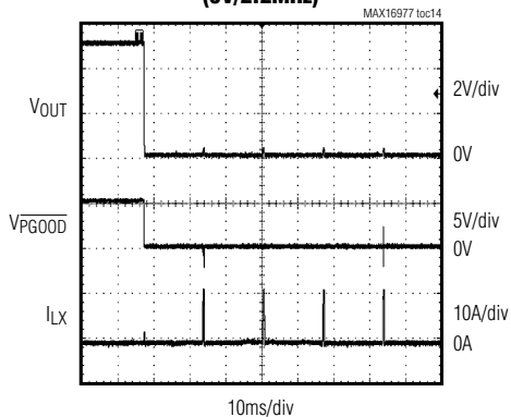
SHORT CIRCUIT TO GROUND TEST (5V/2.2MHz)
