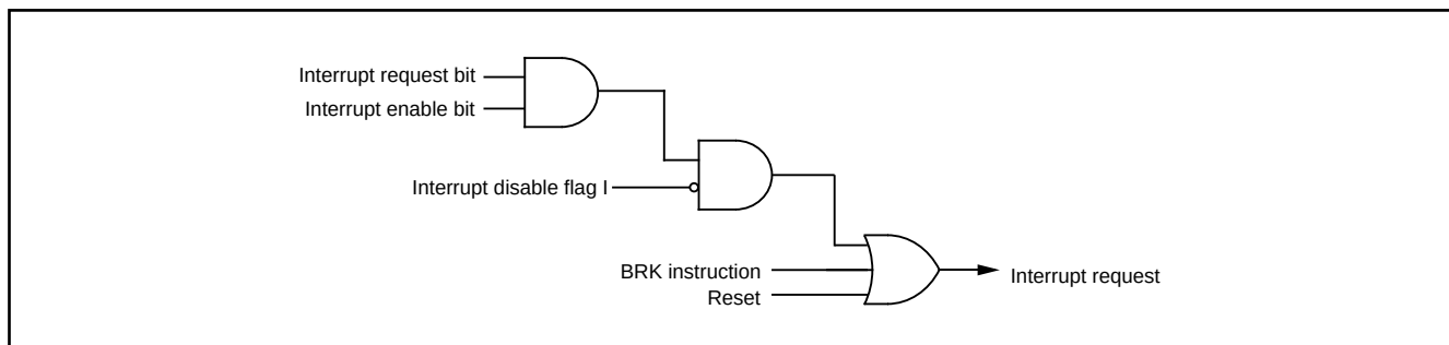
Fig. 14 Interrupt control
