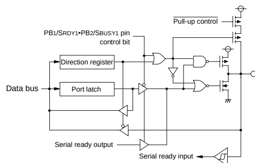
(19) Port PB1
