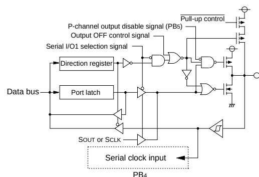
Fig. 13 Port block diagram (3)
