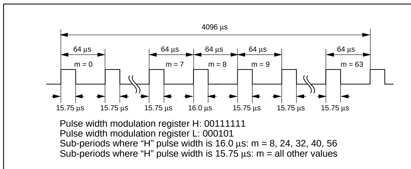
Fig. 65 PWM timing
