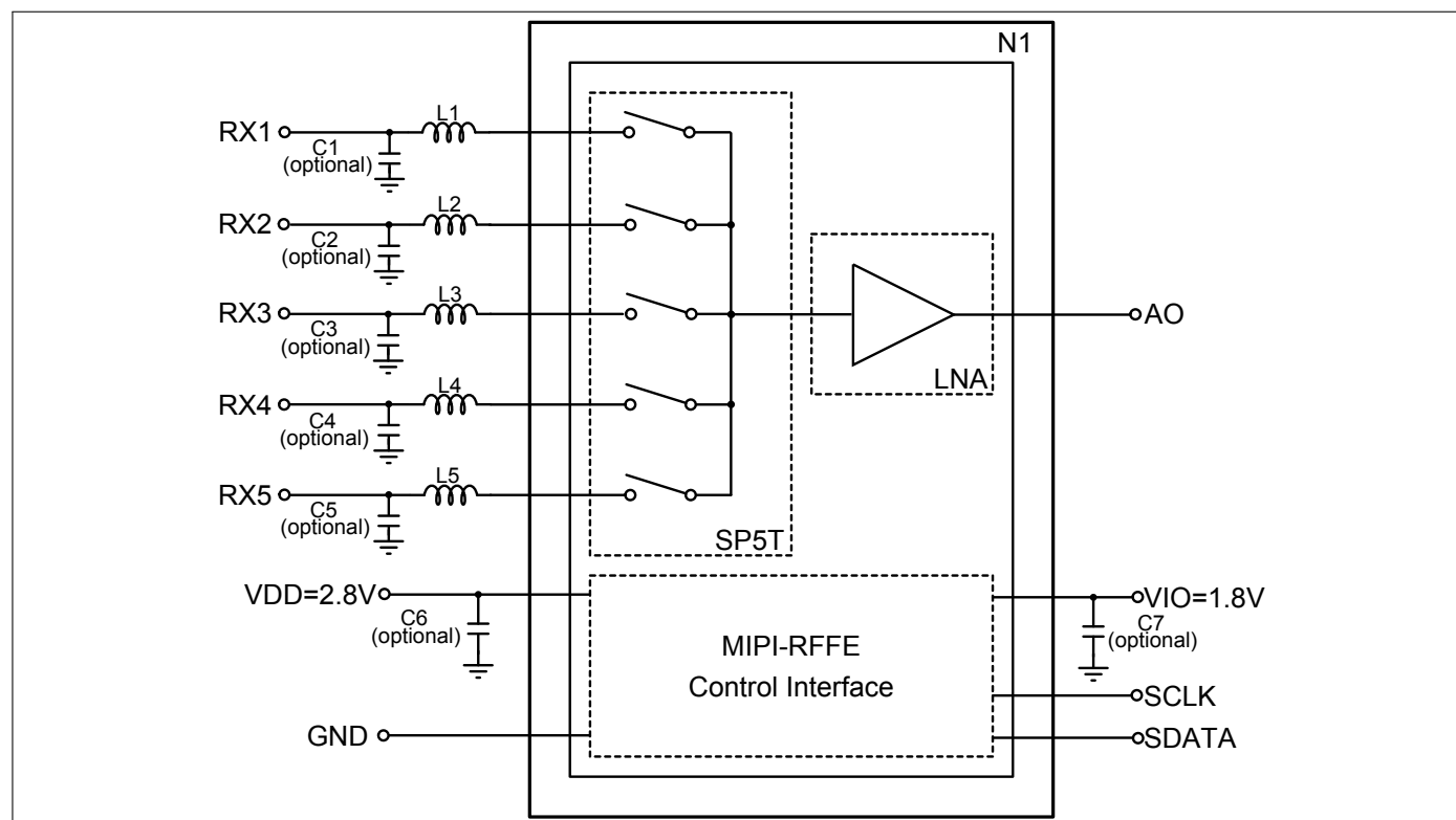
Figure 8: BGM15LA12 Application Schematic
