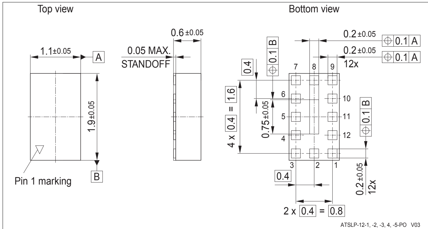
Figure 9: ATSLP-12-1 Package Outline (top, side and bottom views)
