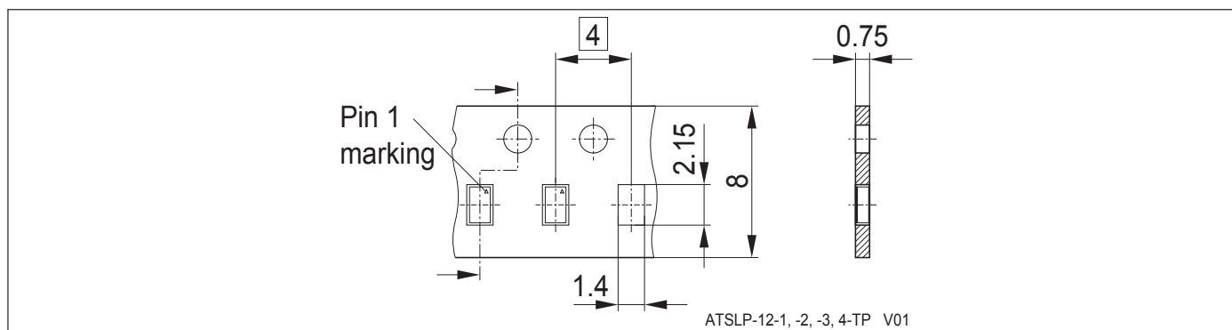
Figure 12: ATSLP-12-1 Carrier Tape
