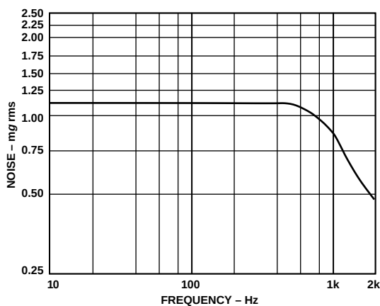
Figure 11. Noise Spectral Density
