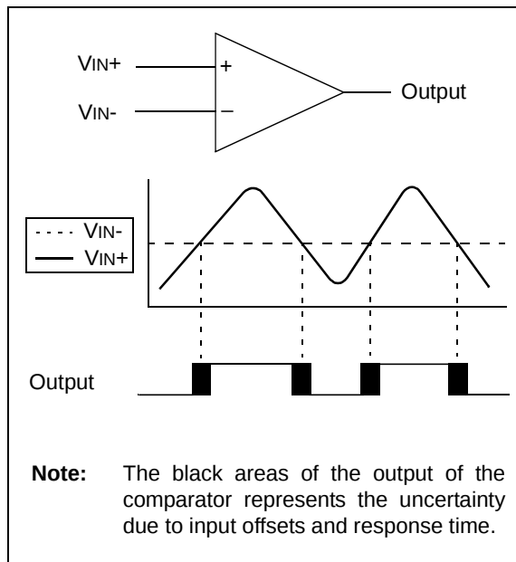
FIGURE 20-1: SINGLE COMPARATOR
