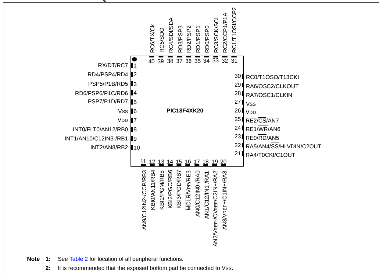
FIGURE 4: 40-PIN UQFN
