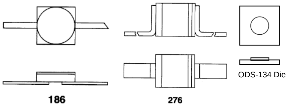
Typical Coplanar Packages
