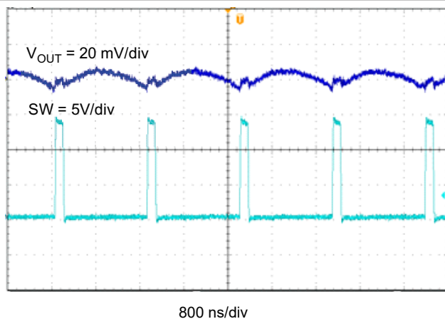
图 8-8. TPS562201 Output Voltage Ripple, I_{OUT} = 0.25 A
