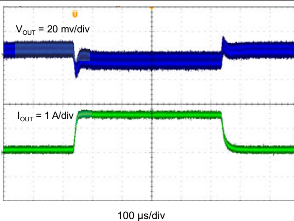
图 8-13. TPS562208 Transient Response 0.1 to 2 A
