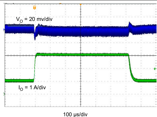
图 8-12. TPS562201 Transient Response, 0.75 to 2.25 A
