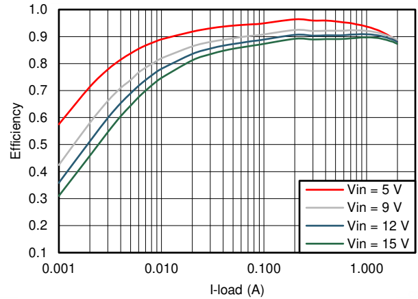
图 6-12. TPS562201 V_{OUT} = 3.3\text{ V} Efficiency, L = 3.3\text{ }\mu\text{H}
