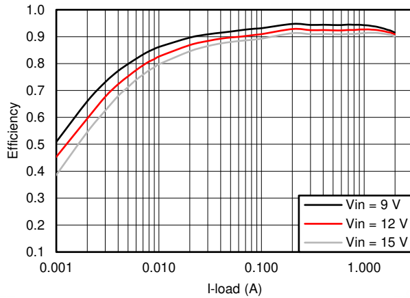
图 6-13. TPS562201 V_{OUT} = 5\text{ V} Efficiency, L = 3.3\text{ }\mu\text{H}
