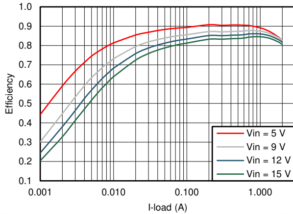
图 6-11. TPS562201 V_{OUT} = 1.8\text{ V} Efficiency, L = 2.2\text{ }\mu\text{H}
