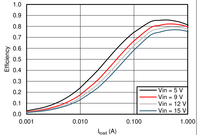
图 6-14. TPS562208 V_{OUT} = 1.05\text{ V} Efficiency, L = 2.2\text{ }\mu\text{H}
