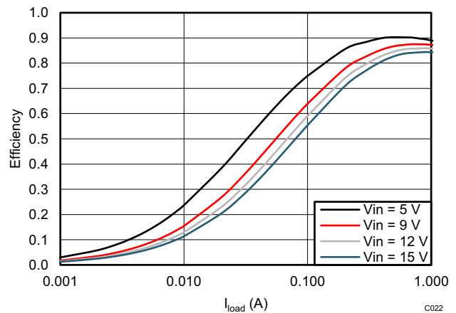
图 6-16. TPS562208 V_{OUT} = 1.8\text{ V} Efficiency, L = 2.2\text{ }\mu\text{H}
