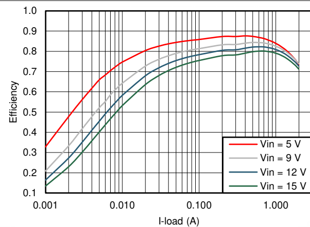
图 6-9. TPS562201 V_{OUT} = 1.05 V Efficiency, L = 2.2 \mu H
