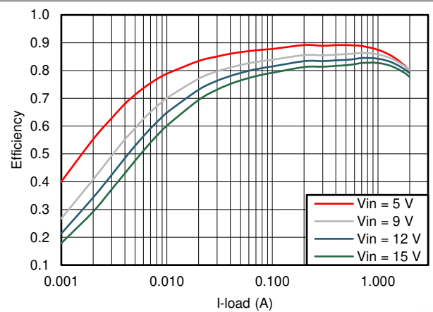
图 6-10. TPS562201 V_{OUT} = 1.5 V Efficiency, L = 2.2 \mu H
