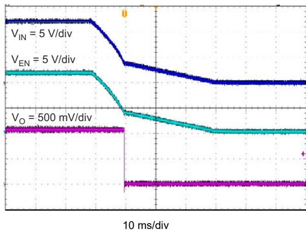
图 8-16. TPS562201 Shutdown Relative to V_I
