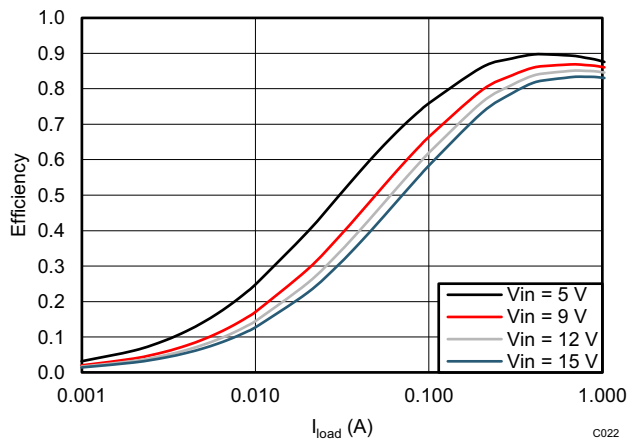
图 6-15. TPS562208 V_{OUT} = 1.5\text{ V} Efficiency, L = 2.2\text{ }\mu\text{H}
