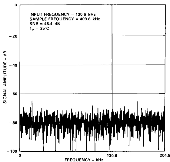
Figure 14. ADC FFT Plot
