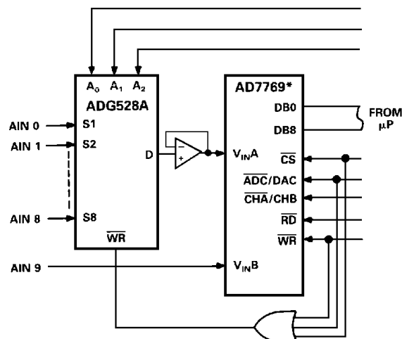
Figure 31. Multichannel Inputs
