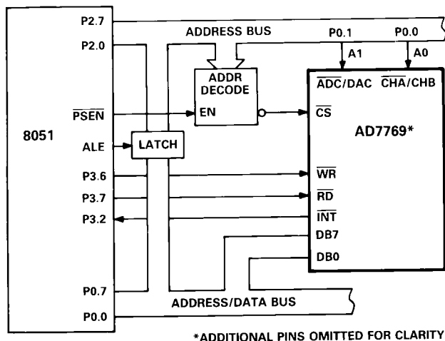
Figure 20. AD7769 to 8051 (Processor Bus) Interface
