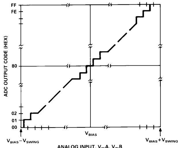
Figure 5. ADC Transfer Function
