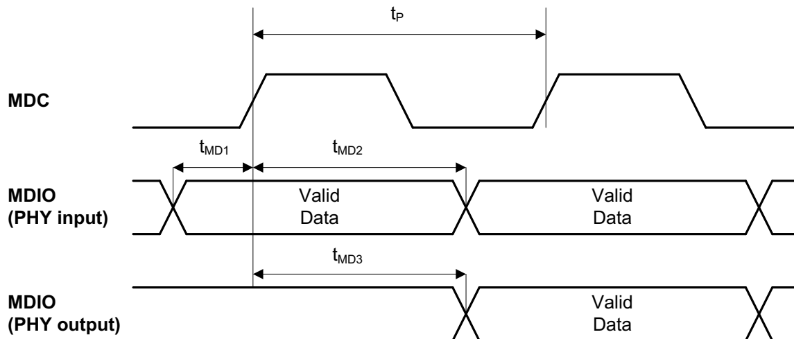
Figure 21. MDC/MDIO Timing
