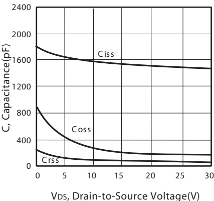
Figure 9. Capacitance
