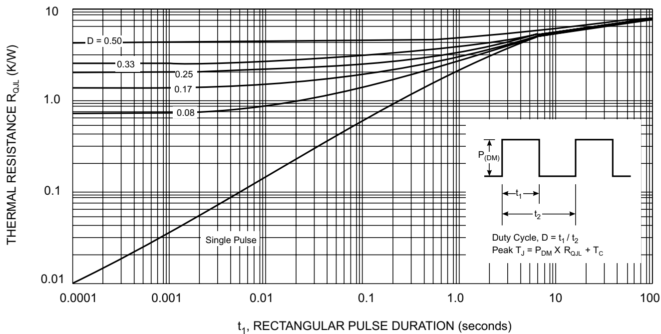
Fig. 5, Typical Thermal Resistance R_{QJL}
