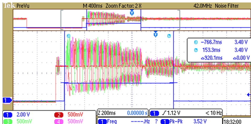
Figure 8. Open-Loop Acceleration
