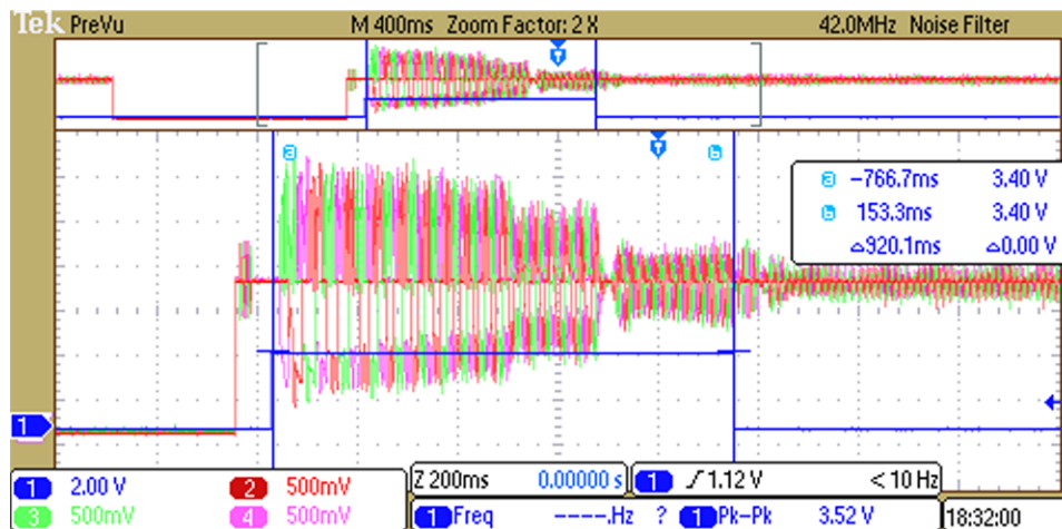
Figure 4. Open-Loop to Closed-Loop Threshold
