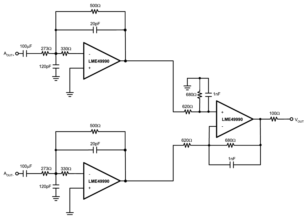
Figure 30. MFB 3rd Order PCM LPF
