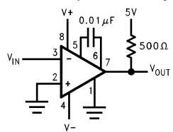
Test Circuit 3 (Collector Output)
