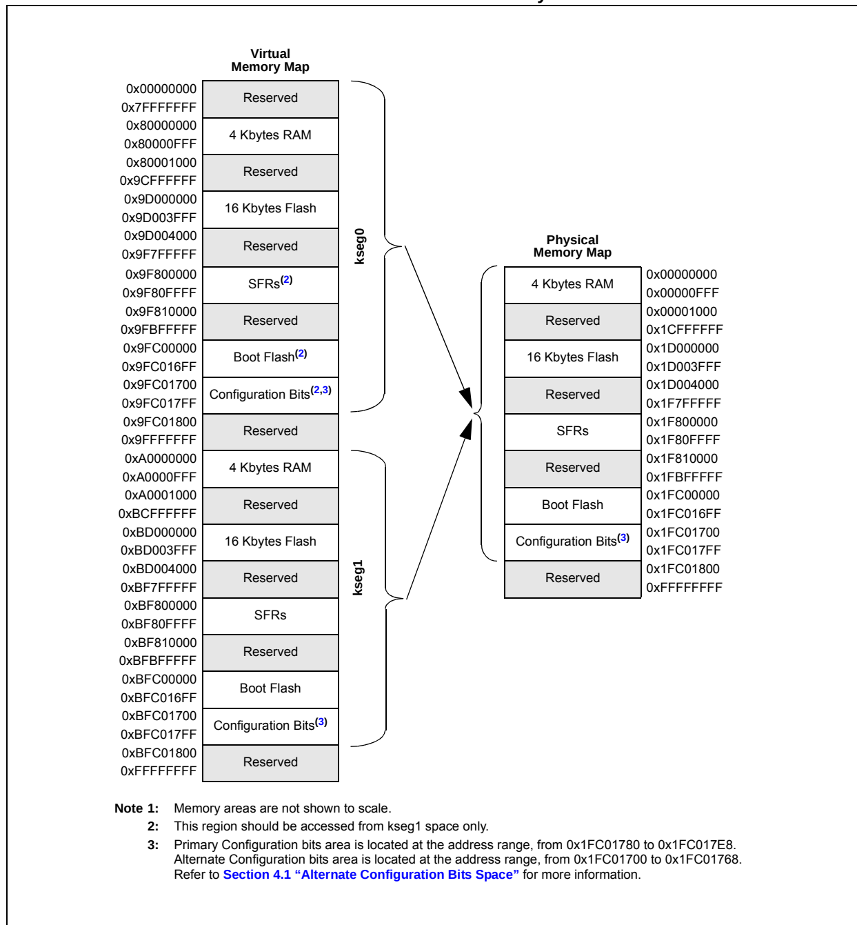
FIGURE 4-1: MEMORY MAP FOR DEVICES WITH 16 Kbytes OF PROGRAM MEMORY (1)
