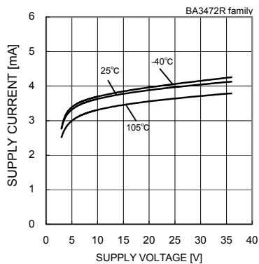
Fig.48 Supply Current - Supply Voltage
