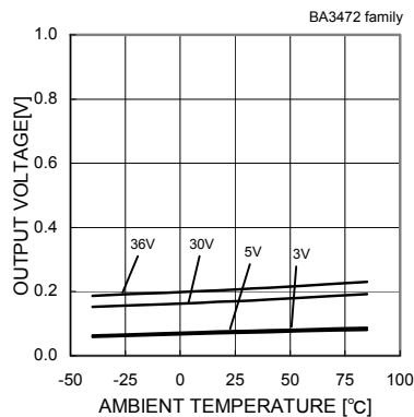
Fig.7 Low level Output Voltage - Ambient Temperature ( R_L=10[k\Omega] )
