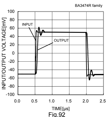
Fig.92 Input / Output Voltage - Time (VCC/VEE=15[V]/-15[V], Av=0[dB], RL=2[kΩ], CL=100[pF], Ta=25[°C])
