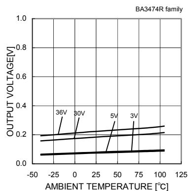
Fig.76 Low level Output Voltage - Ambient Temperature ( R_L=10[k\Omega] )
