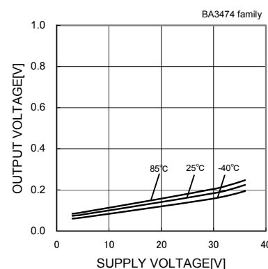
Fig.29 Low level Output Voltage - Supply Voltage ( R_L=10[k\Omega] )
