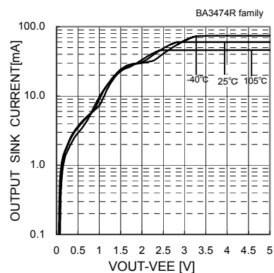
Fig.78 Output Source Current - (VOUT-VEE) ( V_{CC}/V_{EE}=5[V]/0[V] )
