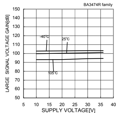
Fig.84 Large Signal Voltage Gain -Supply Voltage
