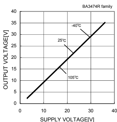
Fig.73 High level Output Voltage - Supply Voltage ( R_L=10[k\Omega] )
