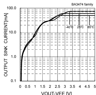
Fig.32 Output Source Current - (VOUT-VEE) ( V_{CC}/V_{EE}=5[V]/0[V] )
