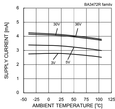
Fig.49 Supply Current - Ambient Temperature
