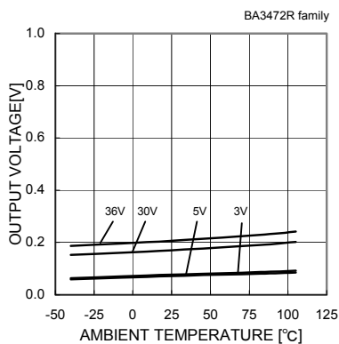
Fig.53 Low level Output Voltage - Ambient Temperature ( R_L=10[k\Omega] )
