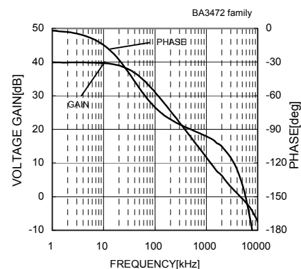
Fig.21 Voltage Gain - Frequency (VCC=7.5[V]/-7.5[V], Av=40[dB], RL=2[kΩ], CL=100[pF], Ta=25[°C])
