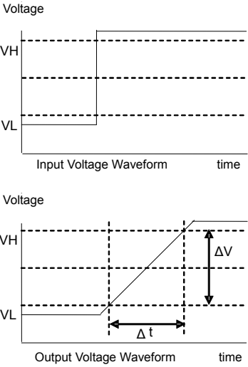
Fig.96 Slew rate input output wave
