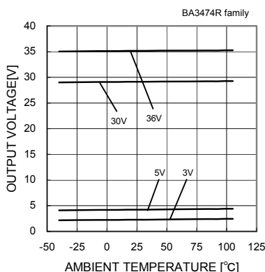
Fig.74 High level Output Voltage - Ambient Temperature ( R_L=10[k\Omega] )
