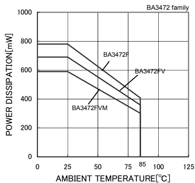
Fig.1 Derating Curve
