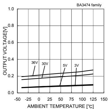
Fig.30 Low level Output Voltage - Ambient Temperature ( R_L=10[k\Omega] )
