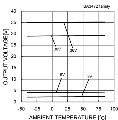
Fig.5 High level Output Voltage - Ambient Temperature ( R_L=10[k\Omega] )
