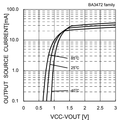
Fig.8 Output Source Current - (VCC-VOUT) ( V_{CC}/V_{EE}=5[V]/0[V] )
