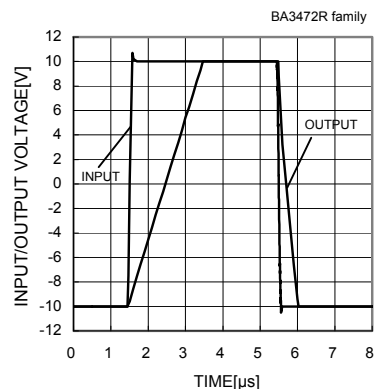
Fig.68 Input / Output Voltage - Time ( V_{CC}/V_{EE}=15[V]/-15[V] , A_v=0[dB] , R_L=2[k\Omega] , C_L=100[pF] , T_a=25[^\circ C] )
