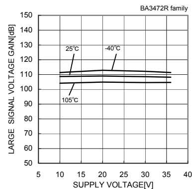
Fig.61 Large Signal Voltage Gain -Supply Voltage
