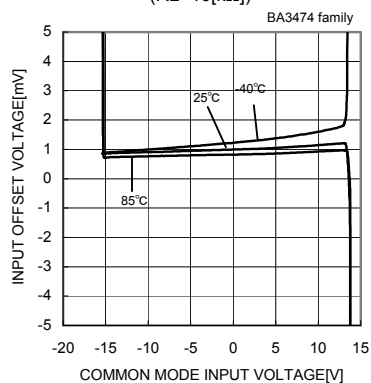
Fig.33 Input Offset Voltage - Common Mode Input Voltage ( V_{CC}/V_{EE}=15[V]/-15[V] )
