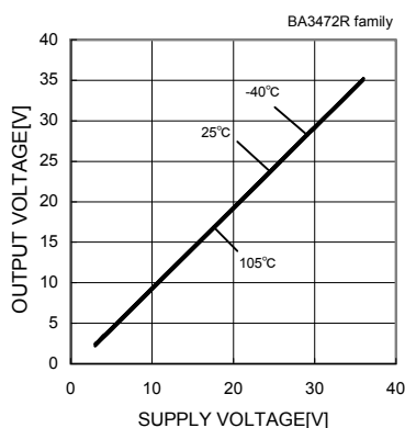
Fig.50 High level Output Voltage - Supply Voltage ( R_L=10[k\Omega] )
