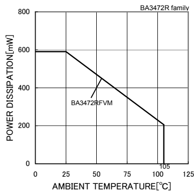
Fig.47 Derating Curve
