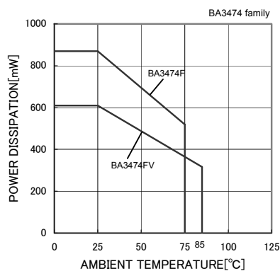
Fig.24 Derating Curve
