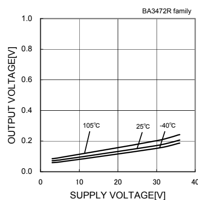
Fig.52 Low level Output Voltage - Supply Voltage ( R_L=10[k\Omega] )
