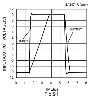
Fig.91 Input / Output Voltage - Time (VCC/VEE=15[V]/-15[V], Av=0[dB], RL=2[kΩ], CL=100[pF], Ta=25[°C])
