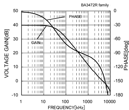
Fig.67 Voltage Gain - Frequency ( V_{CC}=7.5[V] , V_{EE}=-7.5[V] , A_v=40[dB] , R_L=2[k\Omega] , C_L=100[pF] , T_a=25[^\circ C] )
