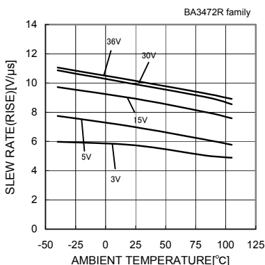
Fig.66 Slew Rate L-H - Ambient Temperature ( R_L=10[k\Omega] )
