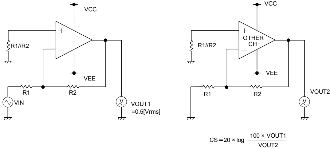
Fig.97 Test circuit 3
