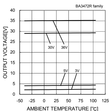
Fig.51 High level Output Voltage - Ambient Temperature ( R_L=10[k\Omega] )
