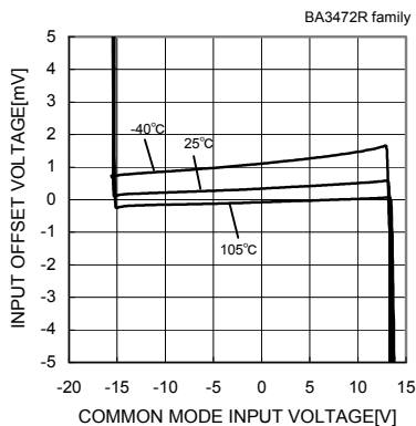
Fig.56 Input Offset Voltage - Common Mode Input Voltage ( V_{CC}/V_{EE}=15[V]/-15[V] )
