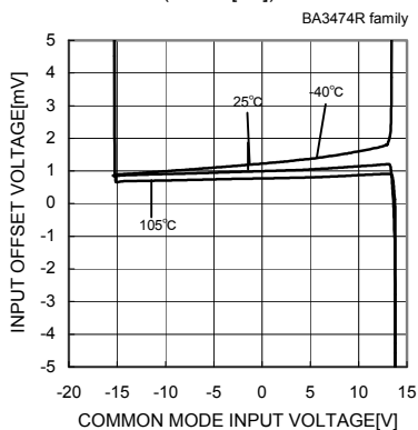
Fig.79 Input Offset Voltage - Common Mode Input Voltage ( V_{CC}/V_{EE}=15[V]/-15[V] )
