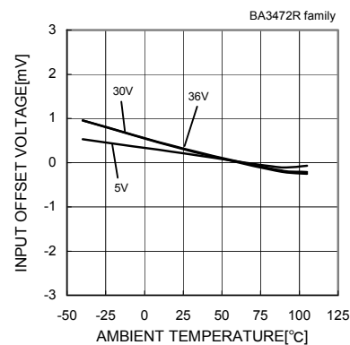
Fig.58 Input Offset Voltage - Ambient Temperature
