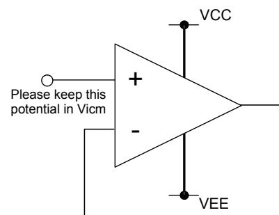
Fig.98 Unused circuit example
