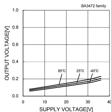
Fig.6 Low level Output Voltage - Supply Voltage ( R_L=10[k\Omega] )
