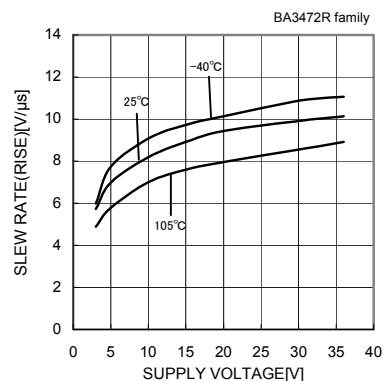
Fig.65 Slew Rate L-H - Supply Voltage ( R_L=10[k\Omega] )
