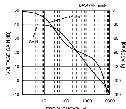
Fig.90 Voltage Gain - Frequency (VCC=7.5[V]/-7.5[V], Av=40[dB], RL=2[kΩ], CL=100[pF], Ta=25[°C])
