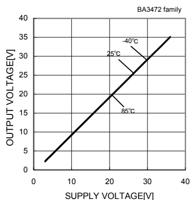
Fig.4 High level Output Voltage - Supply Voltage ( R_L=10[k\Omega] )
