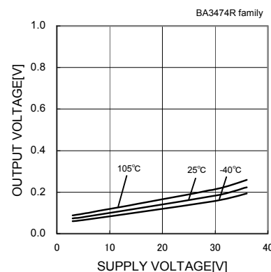
Fig.75 Low level Output Voltage - Supply Voltage ( R_L=10[k\Omega] )
