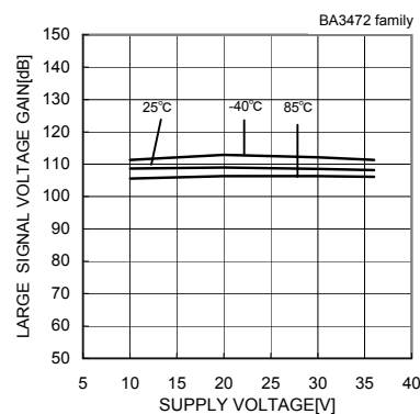
Fig.15 Large Signal Voltage Gain -Supply Voltage
