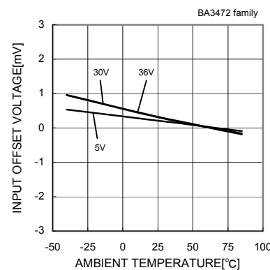
Fig.12 Input Offset Voltage - Ambient Temperature
