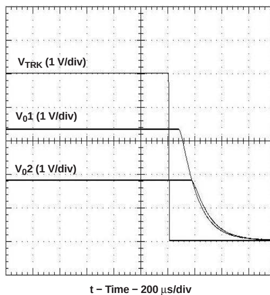
Figure 12. Simultaneous Power Down With Auto-Track Control
