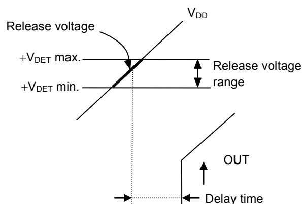
Figure 20 Release Voltage
