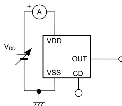
Figure 8 Test Circuit 2
