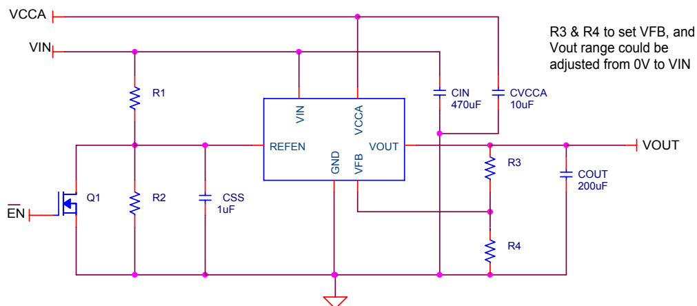
Application Circuit as Adjustable LDO
