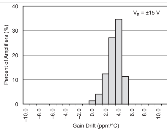
Figure 17. Gain Drift Production Distribution
