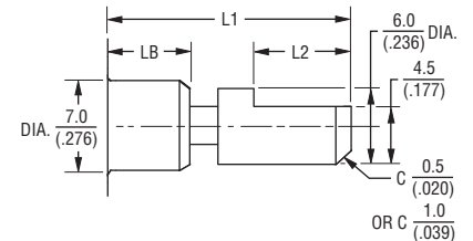
FLATTED SHAFT
