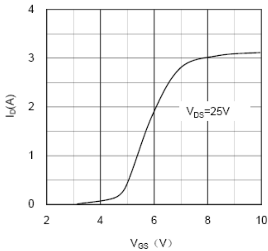
Figure 1. Transfer characteristics
