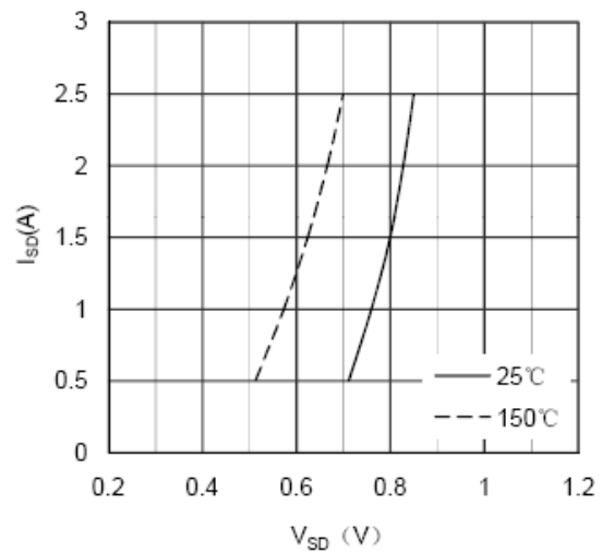
Figure 4. Source-Drain Voltage
