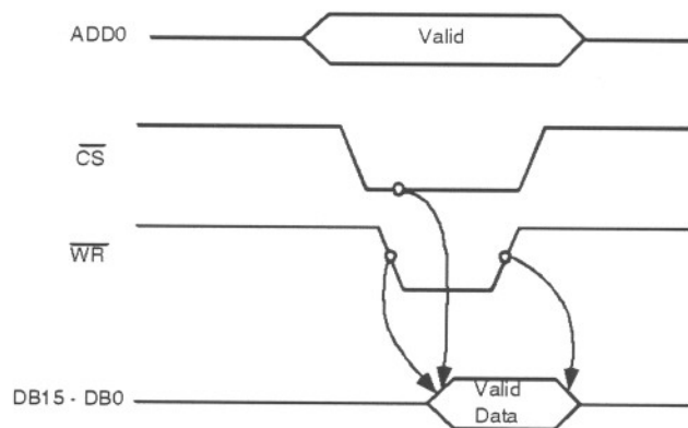
Figure 12. Typical Write Timing
