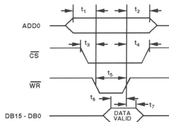
Figure 2. Write Timing Diagram
