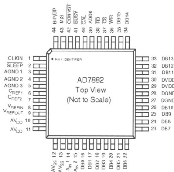
PQFP PINOUT
