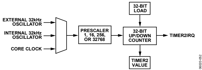
Figure 57. Timer2 Block Diagram
