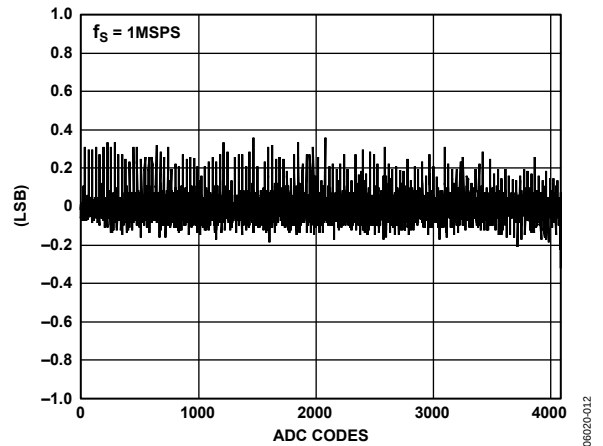
Figure 16. Typical DNL Error, f_s = 1 \text{ MSPS}
