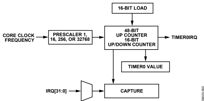
Figure 55. Timer0 Block Diagram
