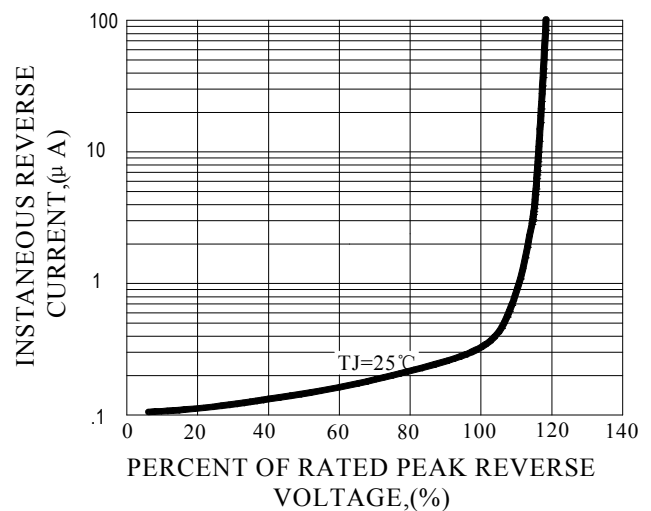
FIG.4-TYPICAL REVERSE CHARACTERISTICS
