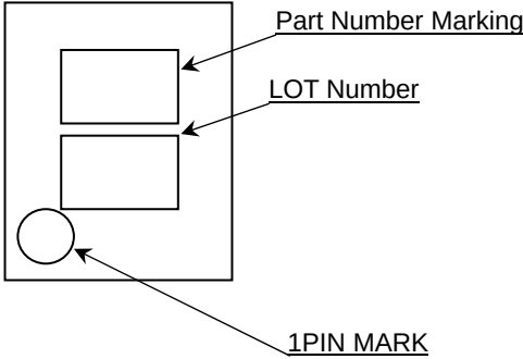
TSSOP-B8(TOP VIEW)
