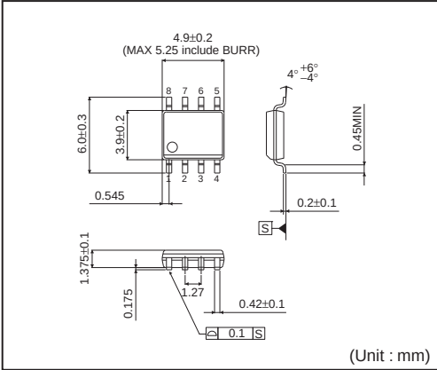
SOP8(TOP VIEW)
