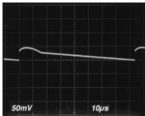
Figure 13. Tantalum Electrolytic
