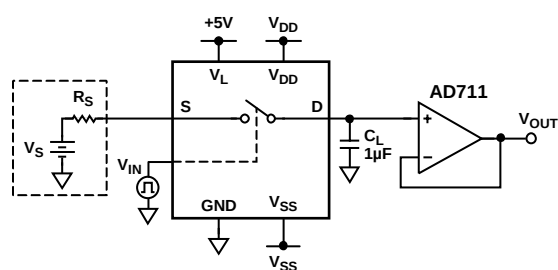
Figure 28. Charge Injection
