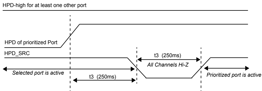
Fig 8. HPD timing
