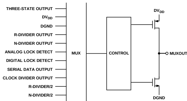
Figure 15. MUXOUT Schematic
