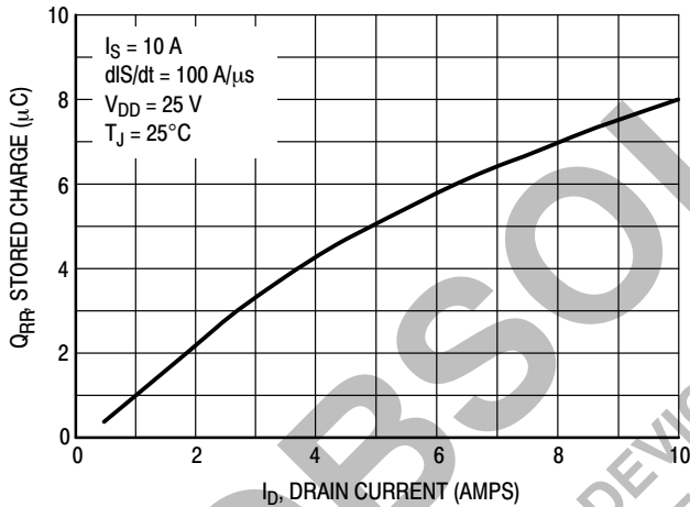
Figure 10. Stored Charge
