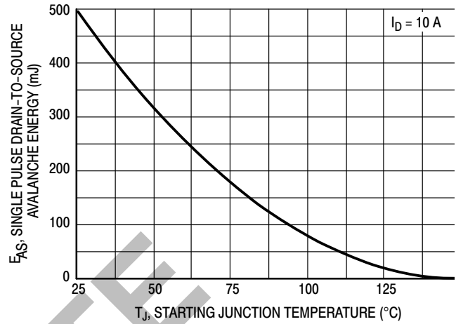
Figure 13. Maximum Avalanche Energy versus Starting Junction Temperature
