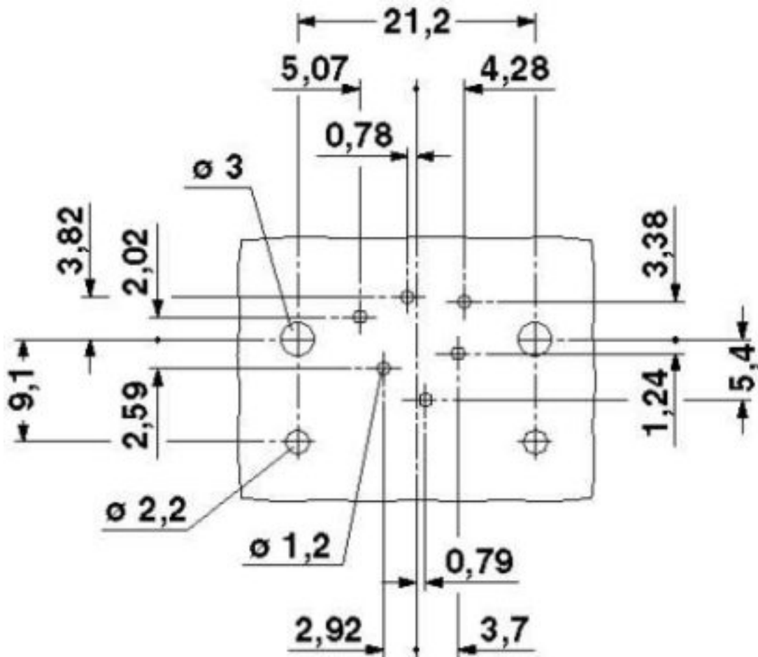
Drilling diagram
