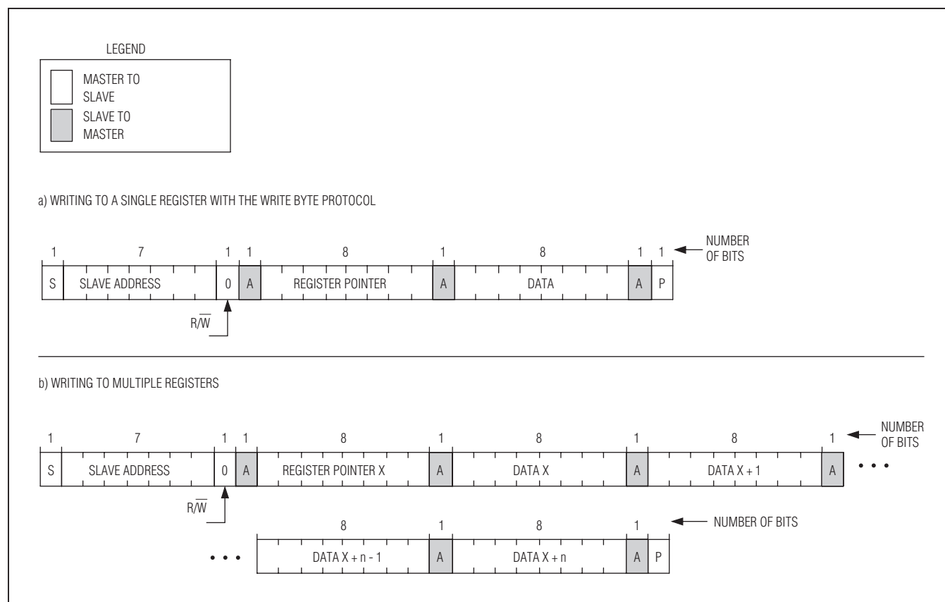
Figure 5. I 2 C Write Operation
