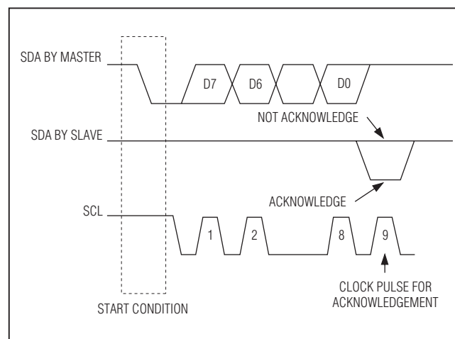
Figure 4. I 2 C Acknowledge
