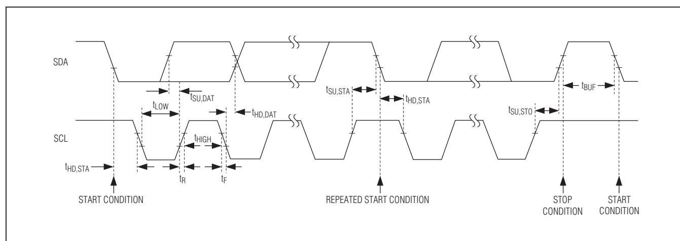
Figure 7. I²C Timing Diagram
