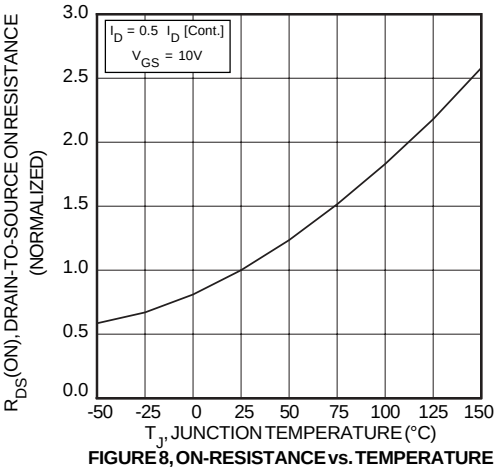
FIGURE 8, ON-RESISTANCE vs. TEMPERATURE
